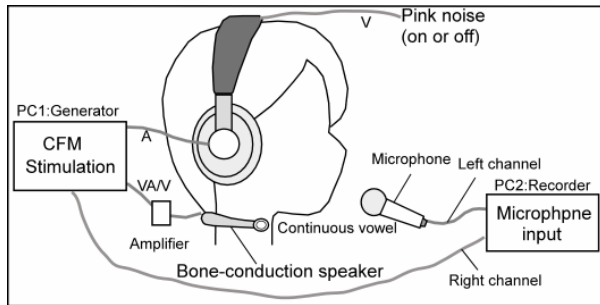
Fig.1. Experimental setup for auditory and vibrotactile stimulation. A paired bone-conduction transducer was fixed near the larynx. PC1 is used to generate composite sinewaves with frequency shifts, and PC2 is used to record produced sounds and stimuli.
