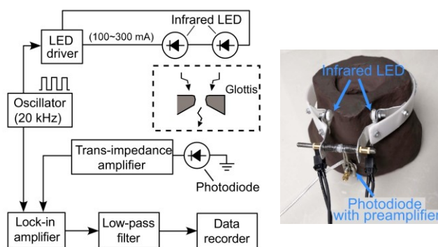
Figure 2, Block diagram of the improved ePGG system with a picture for the component arrangement.
